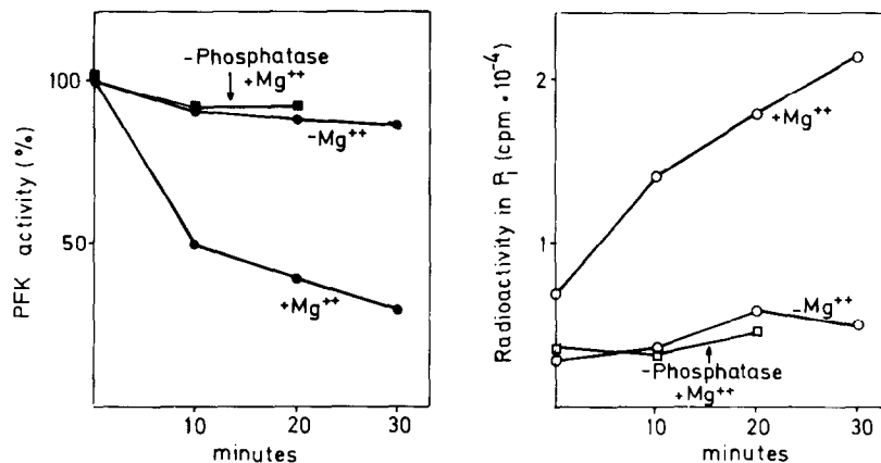
Fig.7. Inactivation of ^{32}\text{P} -labelled active rat liver phosphofructokinase by the inactivating protein (left) and release of free ^{32}\text{P}_i (right). The concentration of \text{MgCl}_2 was 20 mM. Controls contained either 20 mM \text{MgCl}_2 without inactivating protein or inactivating protein but only 0.5 mM \text{MgCl}_2 .
